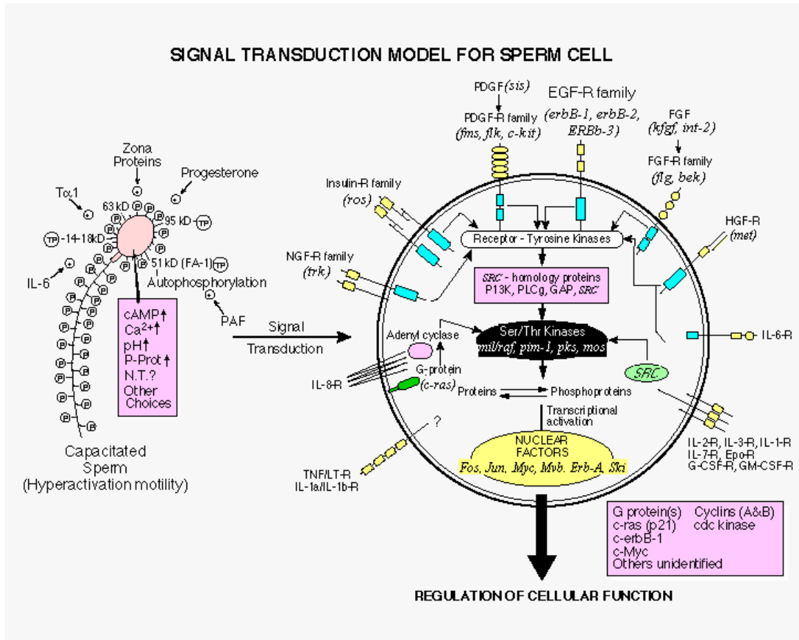
Figure 2 A schematic model for signal transduction in human sperm cell. In a somatic cell, shown in the right circle, the various steps of signal transduction are relatively more defined. Binding of a growth factor/cytokine to sperm leads to phosphorylation/tyrosine phosphorylation of the receptor that activates a cascade of intracellular events leading to elevation of cAMP/cGMP and Ca^{2+} levels. This is followed by induction of transcription and activation/posttranslational modifications of various proteins involved in regulation of cellular function (1-3, 29) The lines with arrows may involve several steps. Hatched rectangles and open circles in the extracellular region of the receptors indicate cysteine-rich and immunoglobulin-like domains, respectively. Filled rectangles in the intracellular region of the receptors show receptor-associated tyrosine kinase domains.
